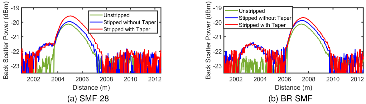
Fig. 6. OTDR of different SMF unstripped (green) stripped without taper (blue) and stripped with taper (red) 25 \mu\text{m} diameter taper between OTDR traces for untapered and tapered fiber. (a) Corning SMF-28 (b) Prysmian Group Bend Resistant SMF.
