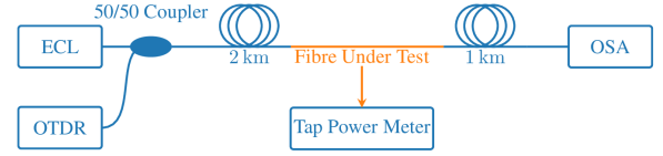
Fig. 4. Experimental setup.
